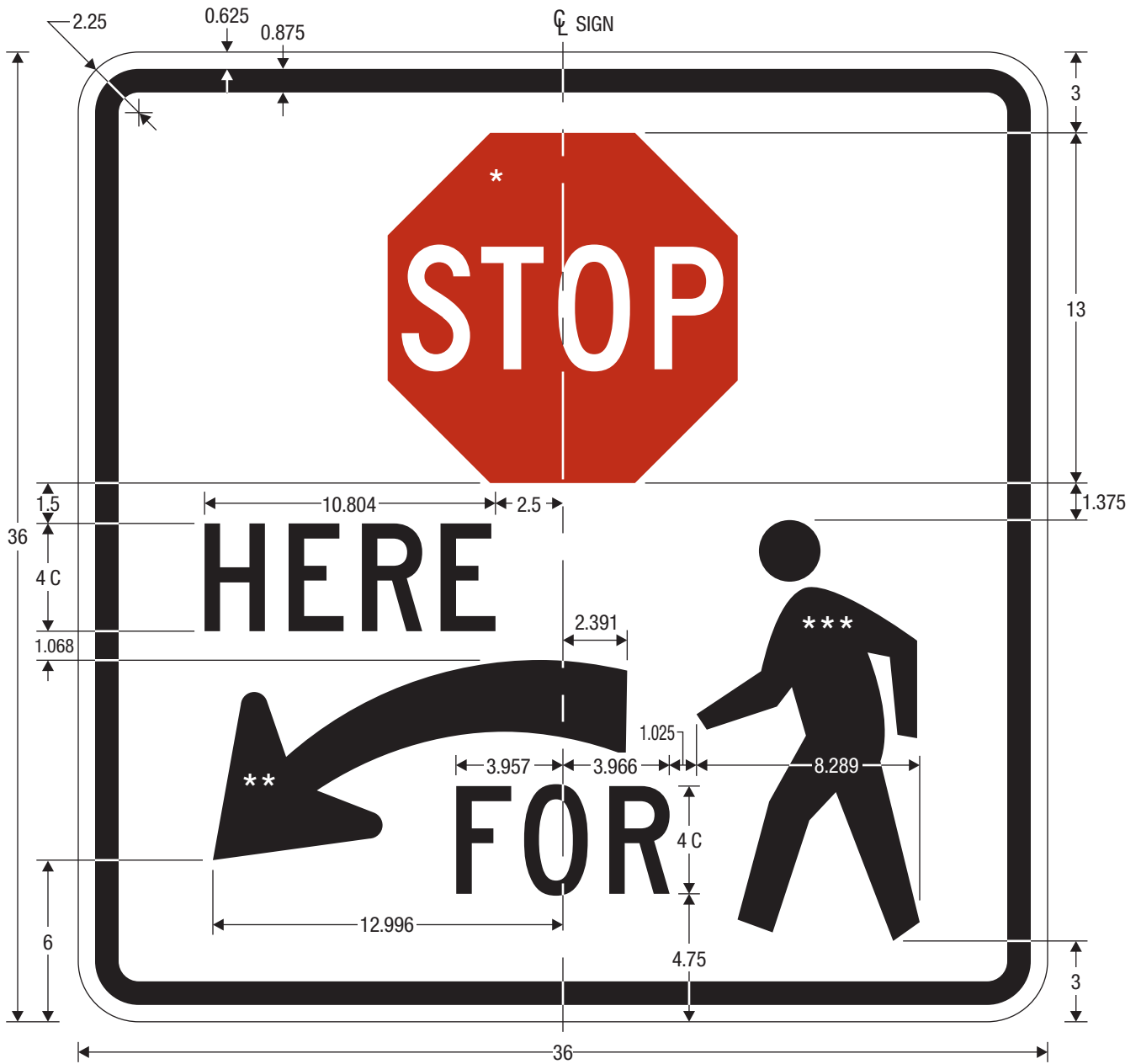
R1-5b STOP HERE FOR PEDESTRIANS (LEFT)
