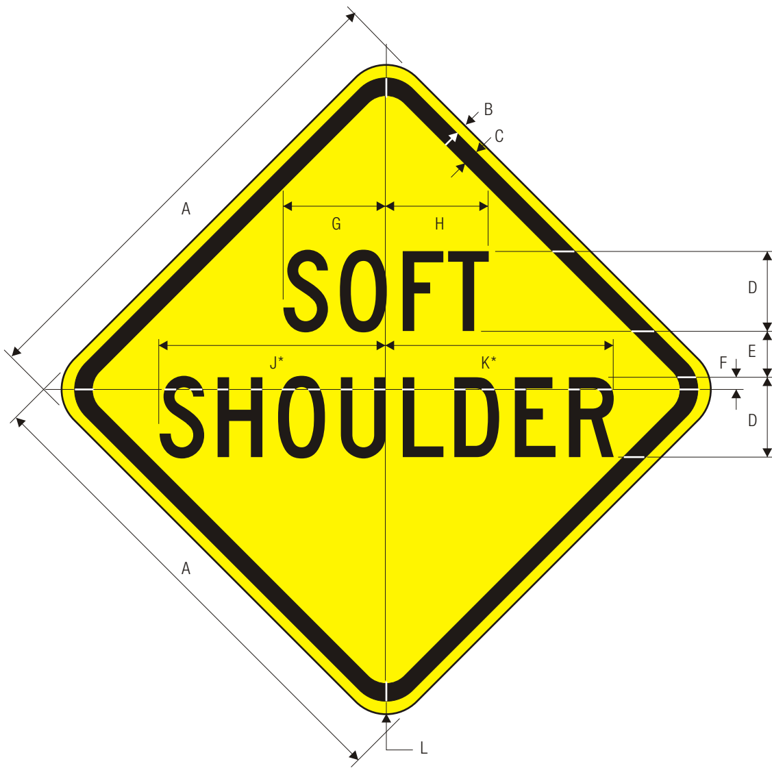
W8-4 SOFT SHOULDER
