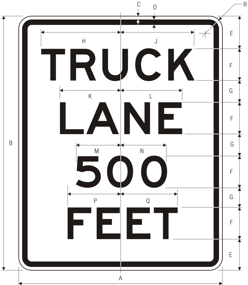
R4-6 TRUCK LANE 500 FEET
