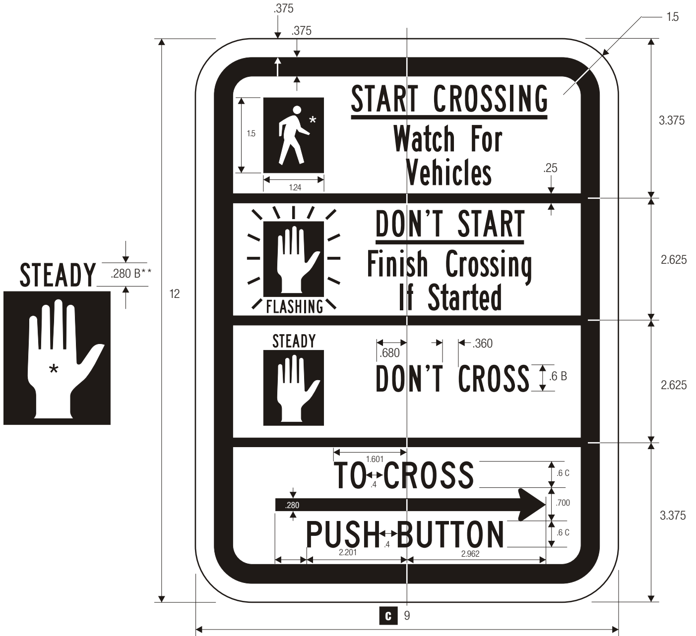
R10-3b PEDESTRIAN TRAFFIC SIGNAL
