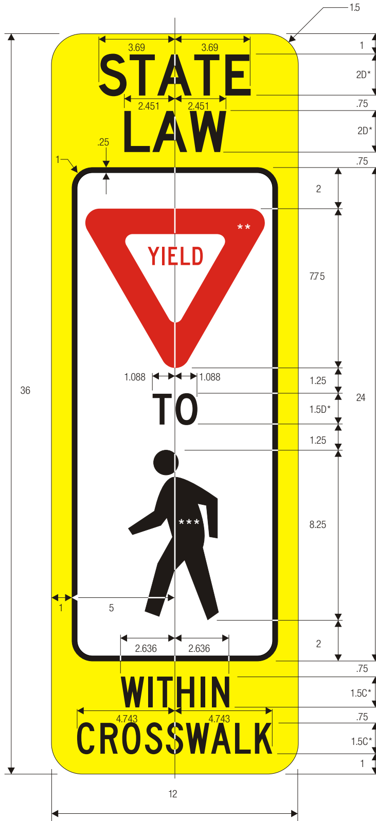
R1-6 IN-STREET PEDESTRIAN CROSSING
